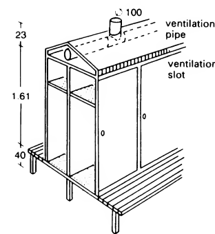
⑩ Lockers with sloping roofs and ventilation pipe
